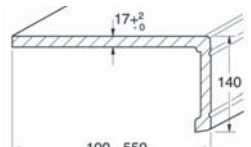
System YF 140
