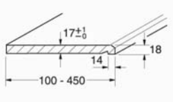
System CF 65
