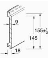
Long profile F
