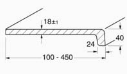
System YF 100
