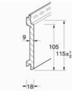
Long profile S
