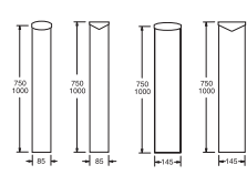
Fence profile S 85 / S 145
