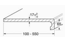
System YF 65
